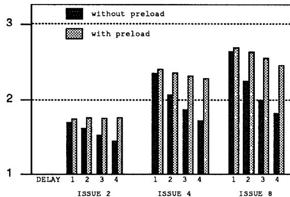
Figure 11: Speedup for Group 1 benchmarks.
