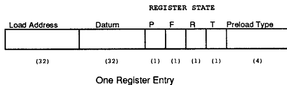
Figure 3: Register states implementation detail.
