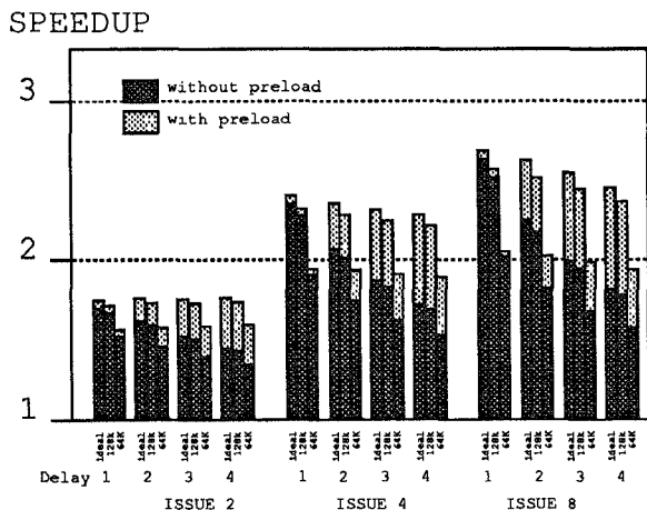
Figure 13: Speedup comparison under cache miss penalty for Group 1 benchmarks.
