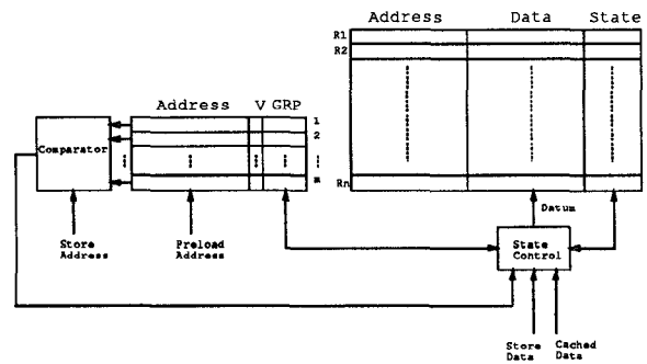
Figure 7: A Subset Design of Preload Register Update.
