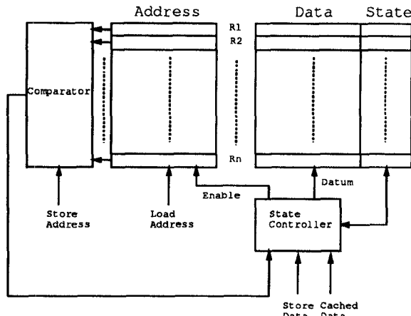
Figure 2: Overview of preload register update.
